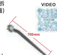
H.C.B-A1199 BENZ (M271) CRANKSHAFT HARMONIC BALANCER PULLEY HOLDER BENZ (M271) 曲軸支撐扳手 (A 271 589 00 40 00)
