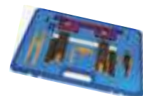
H.C.B-G1188 On car BMW (N55) TIMING TOOL KIT BMW (N55) 正時工具組
